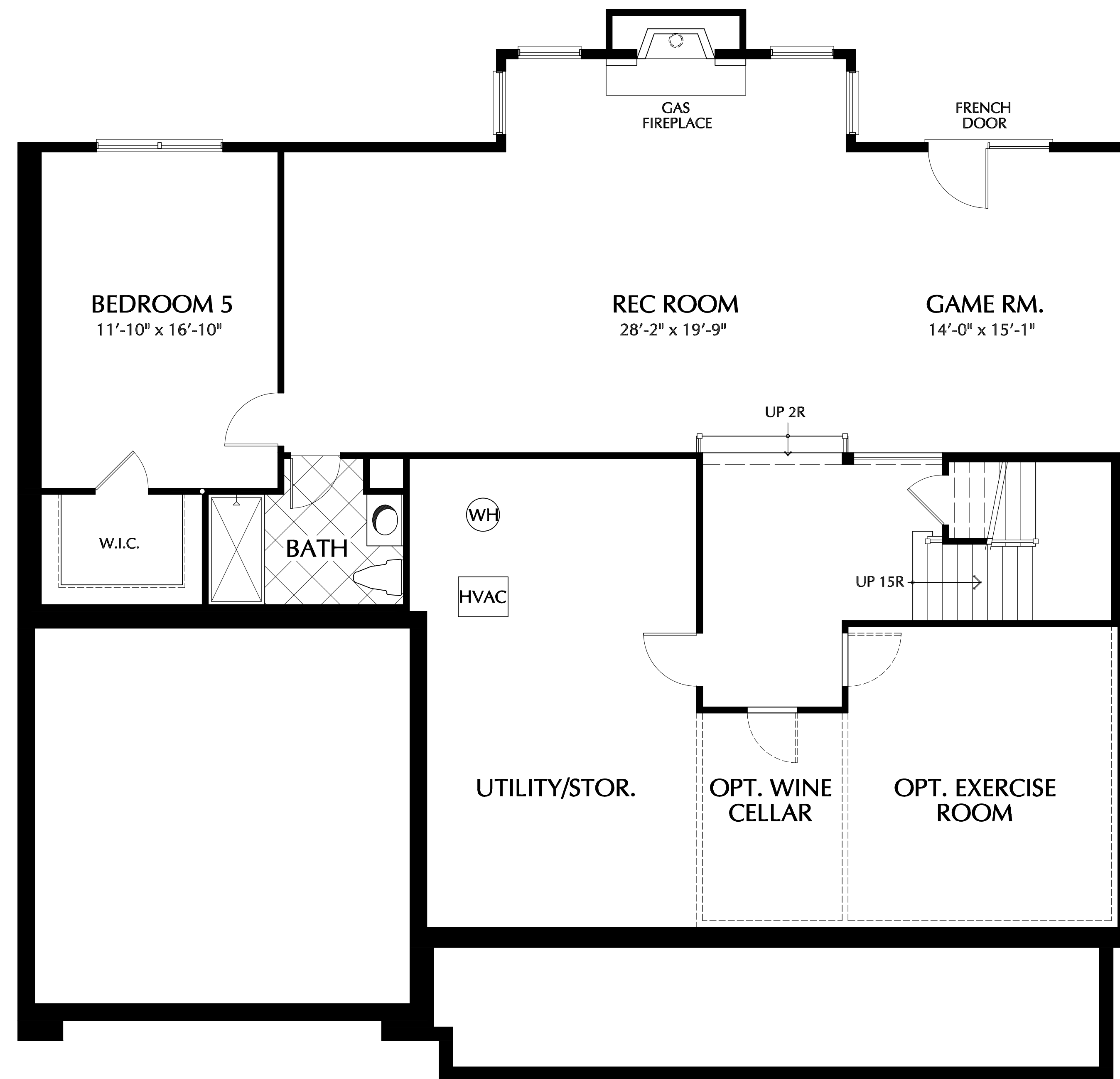
BASEMENT PLAN
